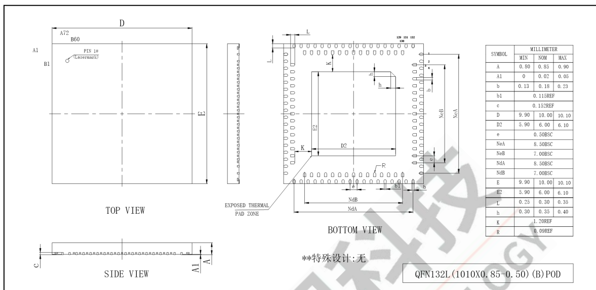
Figure 4-1 AC7926A Package
